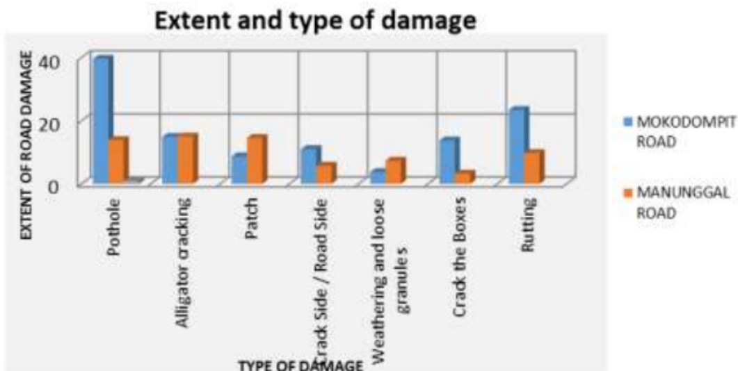
Fig.1. Area and type of road damage
